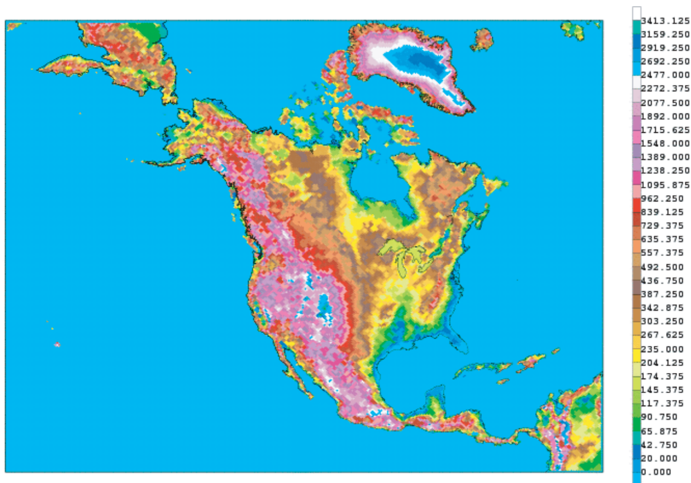
Figure 6.1: North American Regional Reanalysis (NARR) domain and topography.
