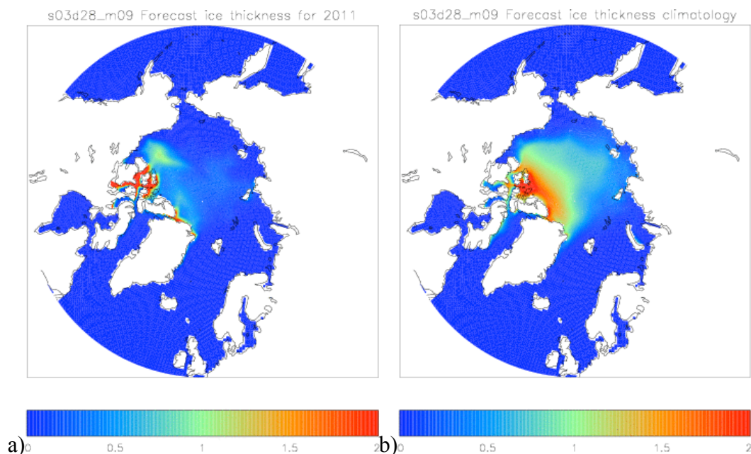
Figure 5. a) Forecast September 2011 ice thickness. b) Hindcast climatological ice thickness. Once again the colour shading saturates at 2m thick ice, but thicker ice does exist.
