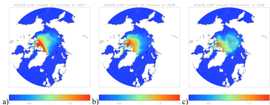
Figure 6. Forecast September ice thickness for a) 2007, b) 2008, and c) 2009. Again the colour shading saturates at 2m thick ice, but thicker ice does exist.
