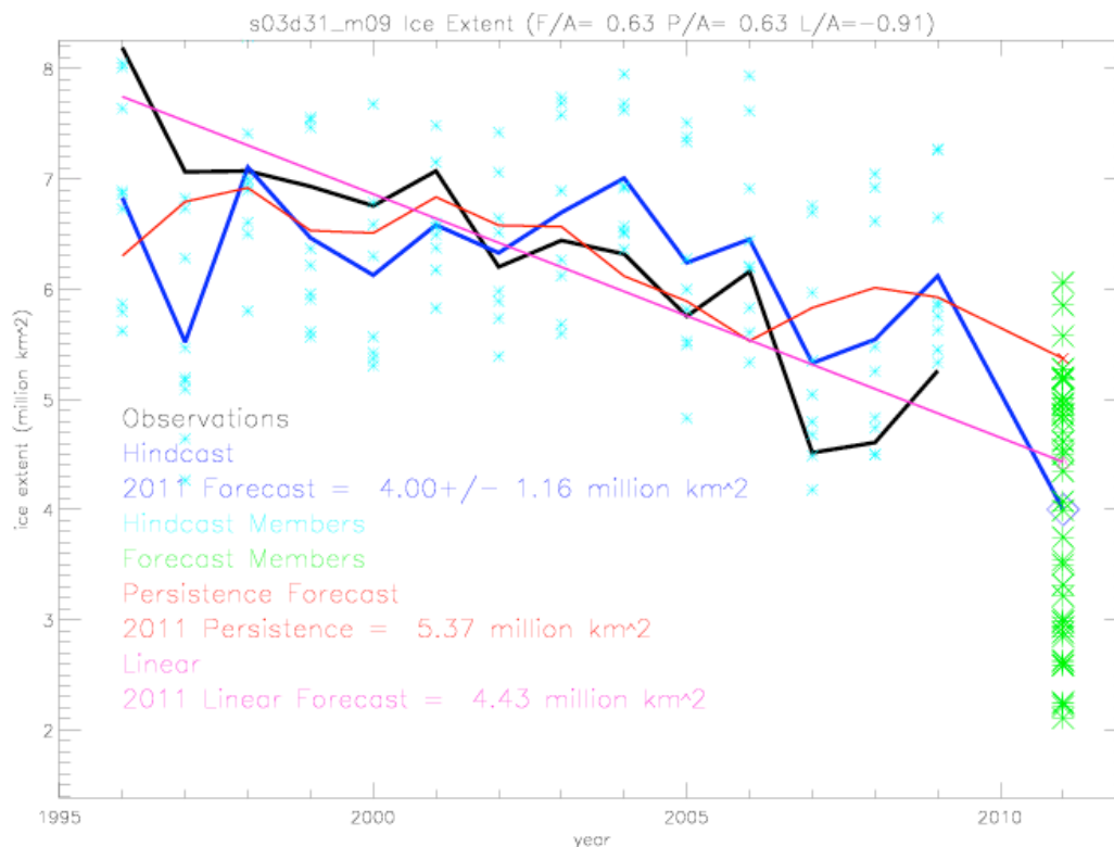
Figure 3: Time series of ice extents for the 1996-2009 hindcast, plus the 2011 forecast. The black line is the observations, and the blue line is the forecast values. The cyan and green x's are the hindcast and forecast ensemble members respectively. Also added to the graph is the persistence forecast (March anomalies added to September climatology) in red and the linear trend in the observations in magenta.
