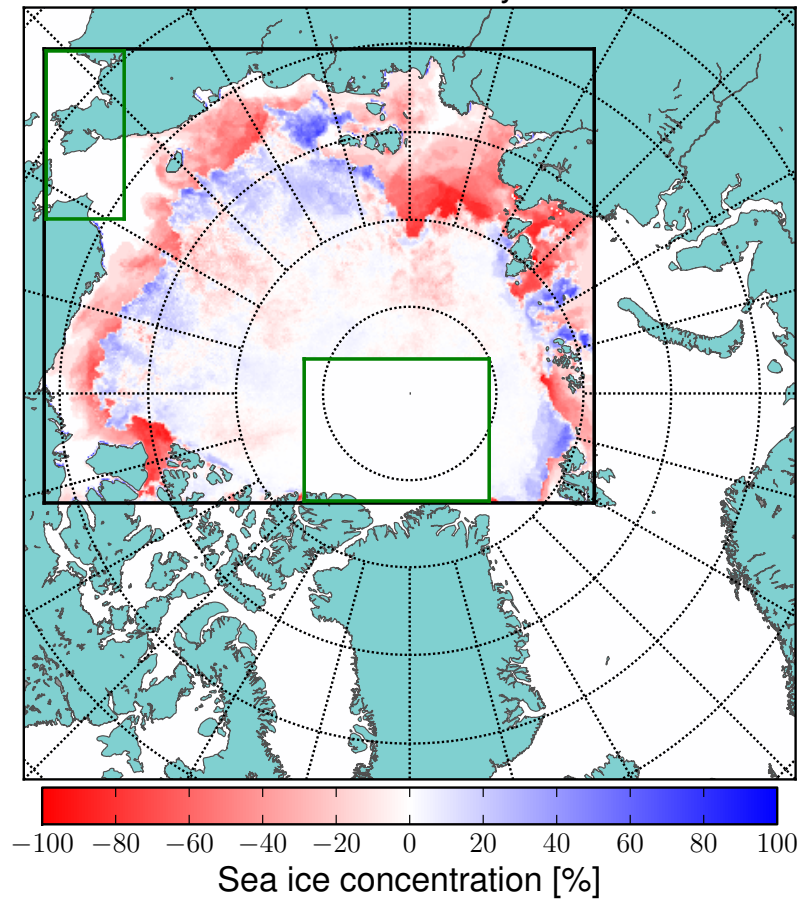
Sea ice concentration anomaly 20110727-0801
