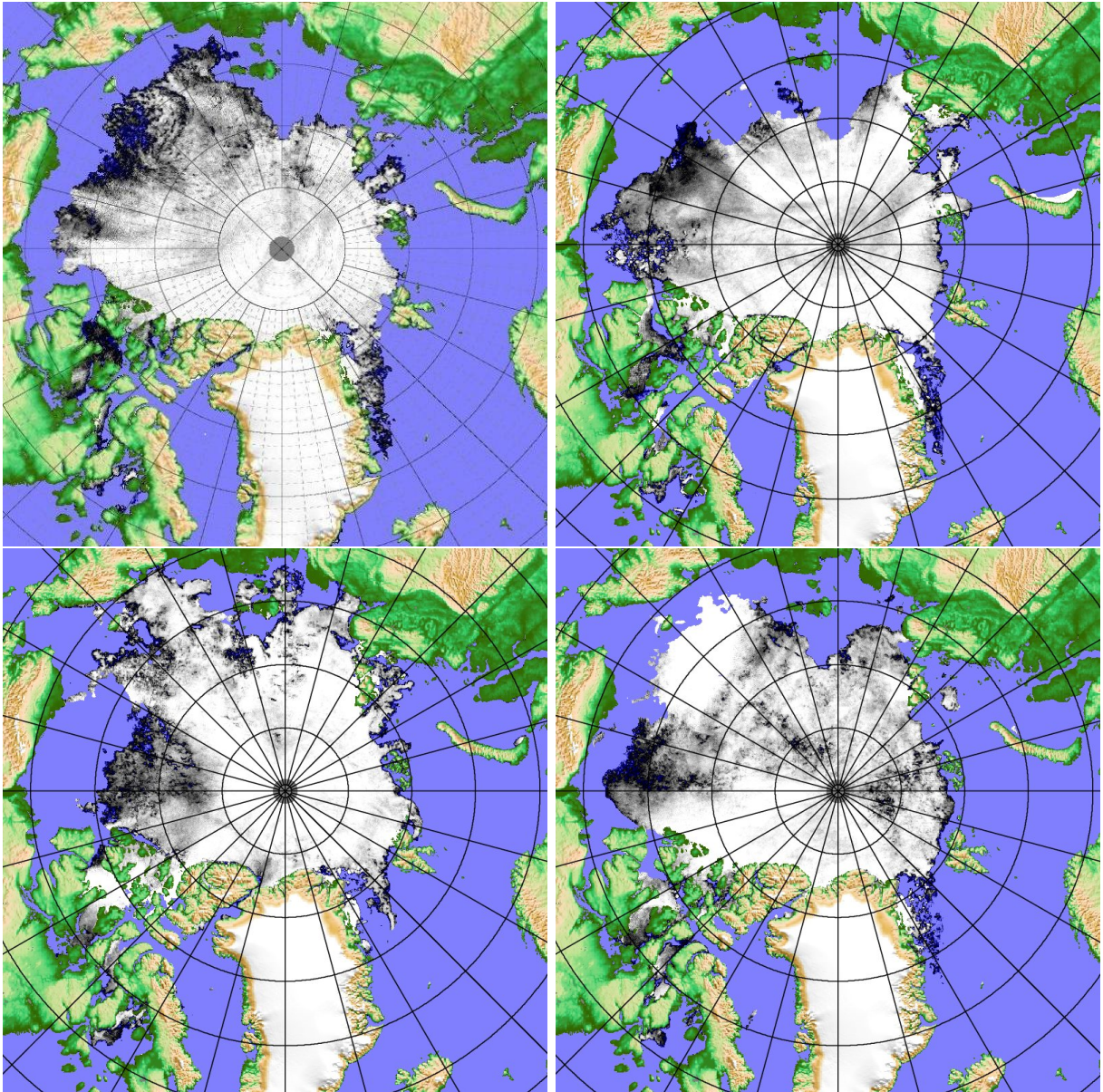
Figure 2: AMSR-E ASI sea ice concentration for August 1 st 2011 (upper left), 2007 (upper right), 2008 (lower left), 2010 (lower right).
