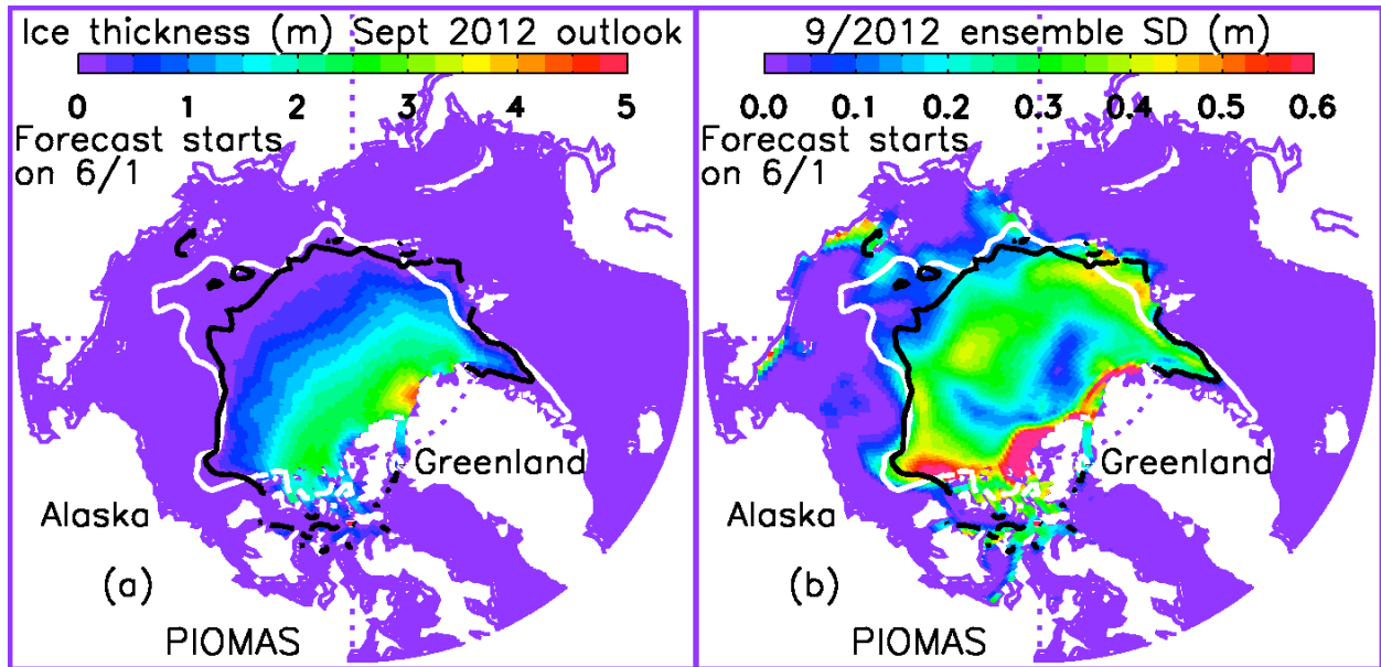
Figure 2. (a) Ensemble median prediction of September 2012 mean sea ice thickness and edge location, and (b) ensemble standard deviation (SD) of ice thickness which shows the uncertainty of the prediction. The white line represents the satellite-observed mean September 2011 ice edge defined as the line of 0.15 ice concentration, while the black line is the model predicted September 2012 ice edge.
