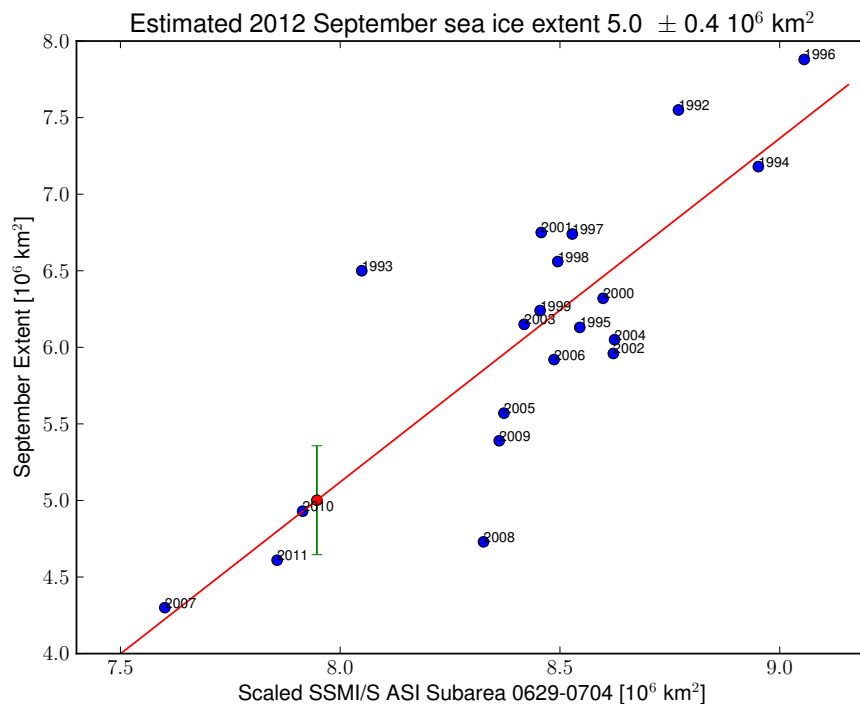
Figure 1: September 2012 sea ice extent estimate.
