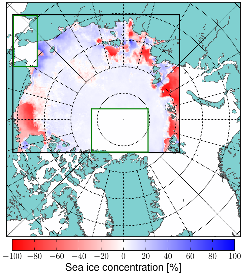
Sea ice concentration anomaly 2012-07-04 (5-day median) w.r.t. 1992-2011 mean
