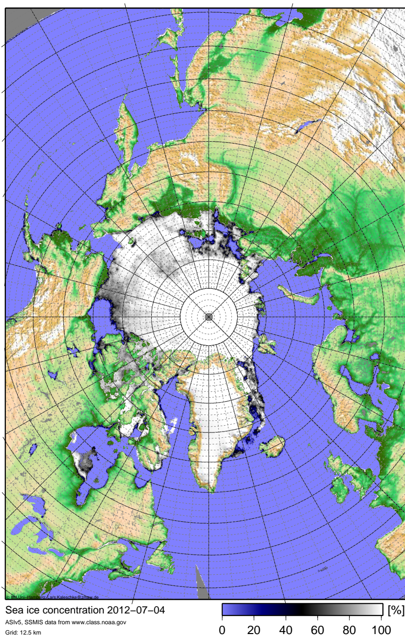
Figure 2: SSMI/S sea ice concentration for July 4, 2012, based on SSMI/S data and processed with ASI algorithm.
