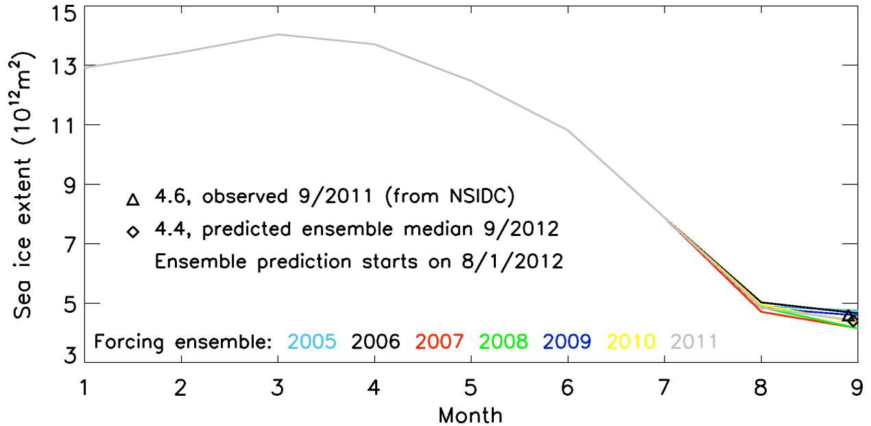
Figure 1. Monthly evolution of arctic sea ice extent from the seven ensemble members. The ensemble median of 4.4 million square km is considered to be the predicted value of arctic sea ice extent for September 2012.
