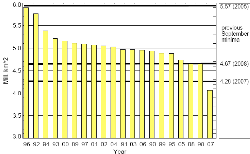
Figure 1. Ensemble I—Simulated mean September ice extent in 2009 [million km 2 ] when forced with atmospheric data from 1989 to 2008 (non-optimized initial state on 11 July 2009). Model derived ice extents have been adjusted by subtracting a bias (see text). The thick black horizontal lines display the minimum ice extents observed in 2005, 2007 and 2008.
