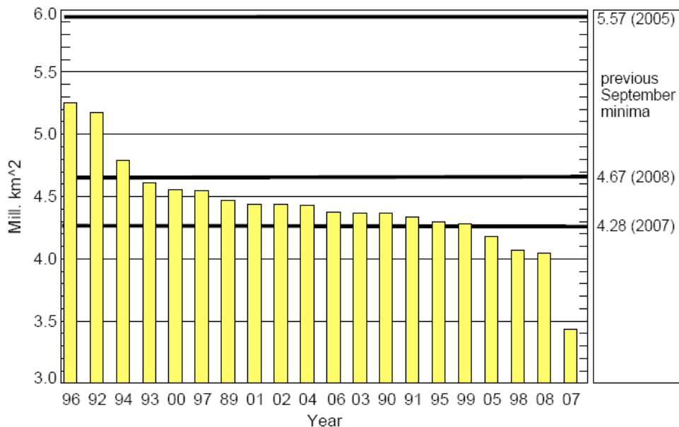
Figure 2. Ensemble II—Simulated mean September ice extent in 2009 [million km 2 ] when forced with atmospheric data from 1989 to 2008 from the optimized initial state on 11 July 2009. The thick black horizontal lines display the minimum ice extents observed in 2005, 2007 and 2008.
