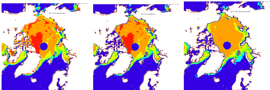
Figure 3: June 1, 2013. Actual observations (left), corrected observations (with the forecast mask applied, center), and forecast based on May 1, 2013, conditions (right). The color scale can be found in figure 2.
