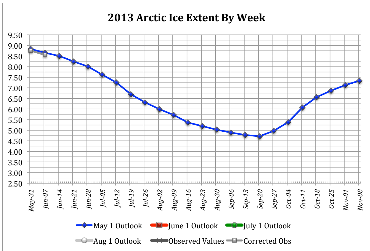
Figure 1: Projected 2013 sea ice extent by week, in millions of square kilometers. The total observed ice extent (SSM/I) on June 1, 2013, was 12.39 million km 2 . A corrected value, removing sea ice in areas where the model does not forecast, such as the Canadian Archipelago, was 8.56 million km 2 for June 1, 2013. The forecast value was 8.83 million km 2 .
