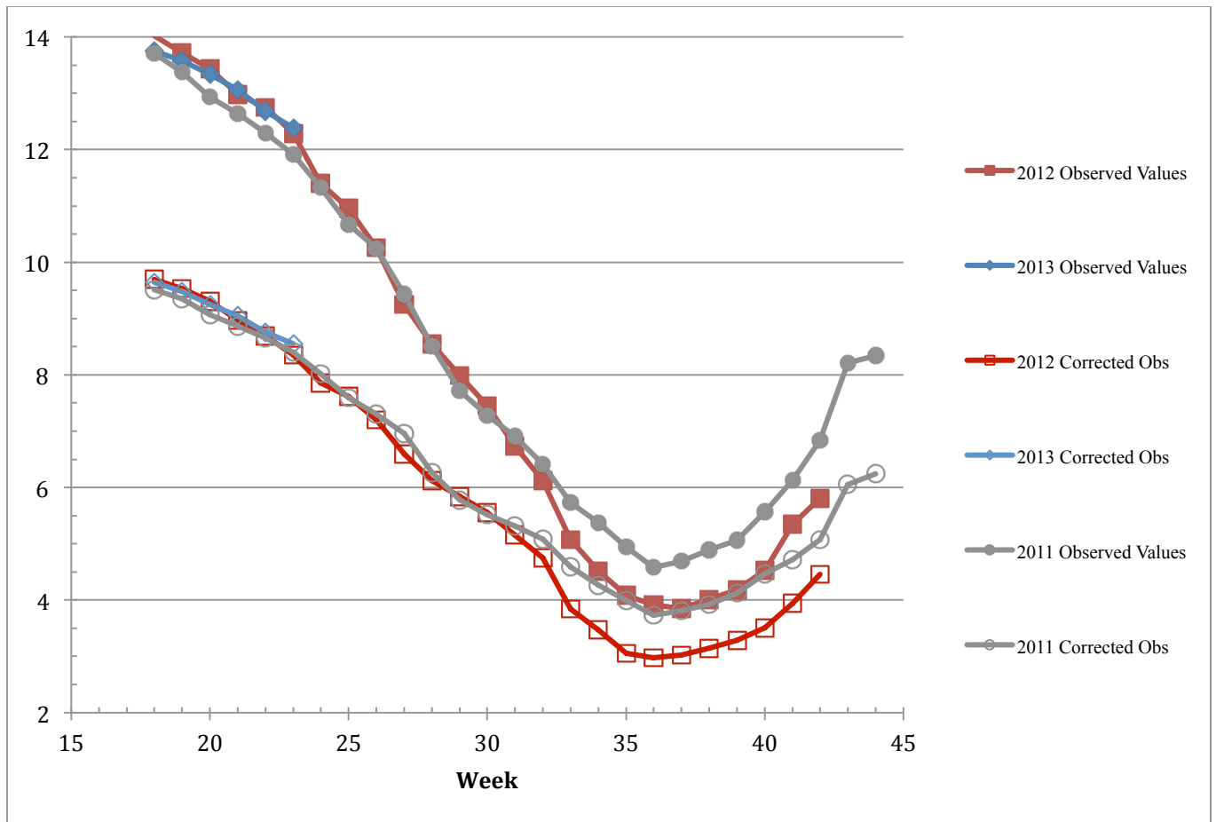
Figure 4: Time-series of observed ice extent (solid shapes) and corrected ice extent (hollow shapes) for summer 2011-2013. 2012 was the lowest summer sea ice extent recorded in the satellite era. 2011 minimum sea ice ice extent was nearly identical in magnitude to the previous record minimum set in September, 2007.
