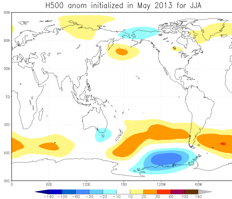
Ensemble-averaged 500 hPa anomalies for the period June-July-August 2013, in geopotential meters.
