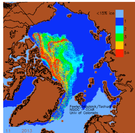
Figure 2. Ice age from week 11 (March ) 2013.
