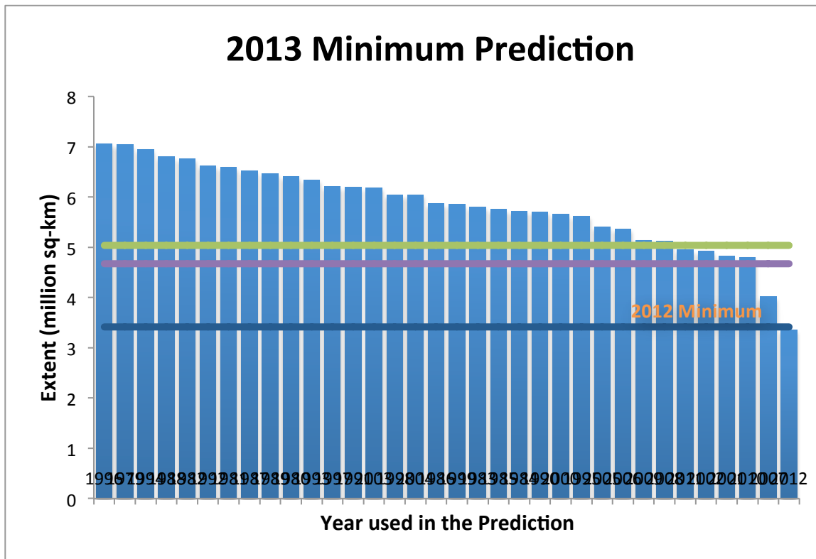
Figure 1. Estimated 2013 minimum extent based on ice age survival rates from previous years (1979-2011). Blue line shows the 2012 September minimum, purple line shows the predicted minimum using an average of the last 5 years of survival rates, whereas the green line shows the predicted minimum using an average of the last 10 years of survival rates.
