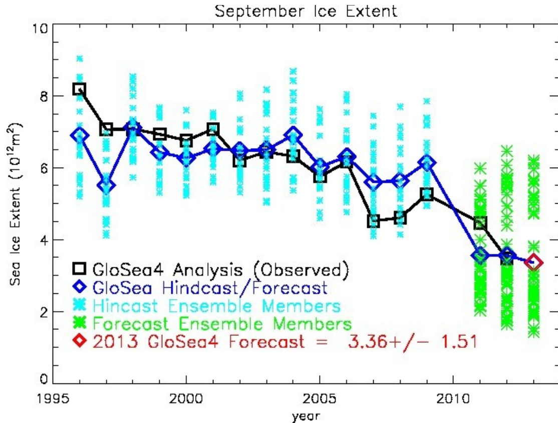
Figure 1: September sea ice extents (million km 2 ) from the GloSea4 seasonal forecasting system, for hindcasts initialised on 25 th March, and 1 st , 9 th , and 17 th April and forecasts initialised between 25 th March and 14 th April. All values (except the observations) have been bias-corrected.
