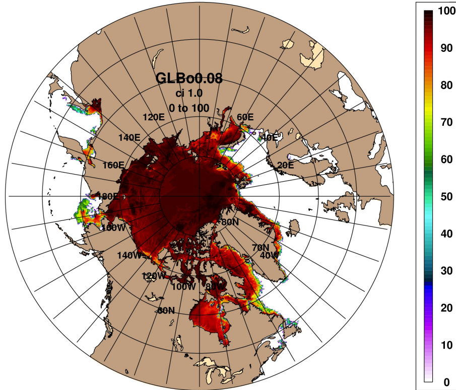
Figure 1: Ice concentration field (%) from GOFS 3.1 valid May 1, 2015. This is the initial condition for each ensemble member.
