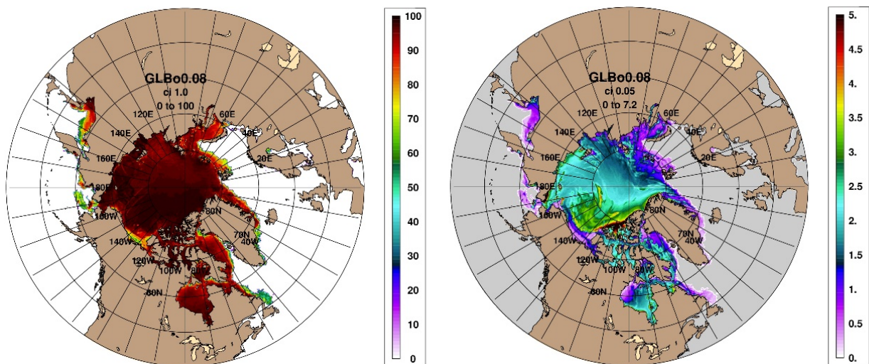
Figure 1: Sea ice concentration (%) and thickness (m) from GOFS 3.1 valid May 1, 2016. These are the initial ice conditions for each ensemble member.
