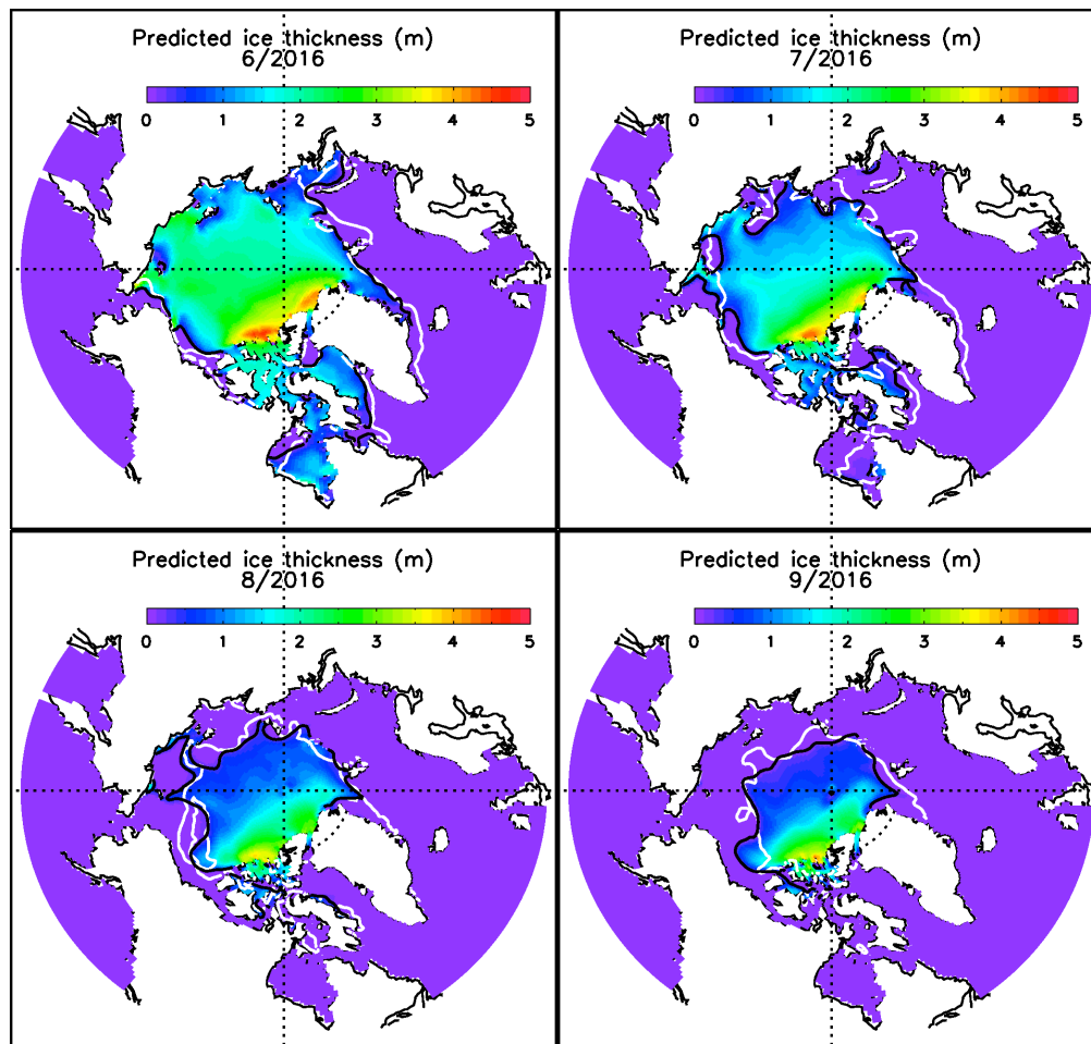
Figure 1. PIOMAS predicted Arctic sea ice thickness for June–September 2016. The white line represents satellite-observed 2015 monthly mean ice edge defined as the contour of 0.15 ice concentration, while the black line is the model predicted 2016 monthly mean ice edge.
