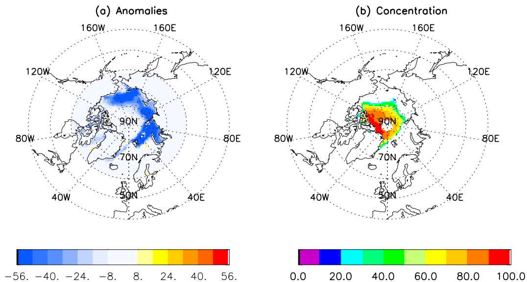
Figure 1 Four-month lead prediction of 2016 September Arctic sea ice concentration anomaly (a) and concentration (b) by the linear Markov model initialized with observed May sea ice concentration, SST and SAT data.
