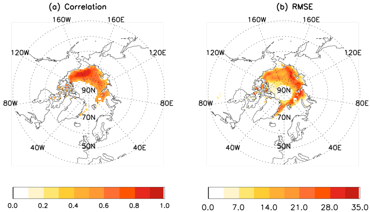
Figure 2. Cross-validated model skills measured by correlations between model predictions and observations of Arctic sea ice concentration anomalies (a) and model RMSE (b) for four-month lead prediction of September sea ice concentration. Only the correlations that pass the 95% confidence level are shown in (a). The units in (b) are in percentages. The low correlations and low RMSE near the North Pole Hole (the satellite blind spot) are due to low ice variability.
