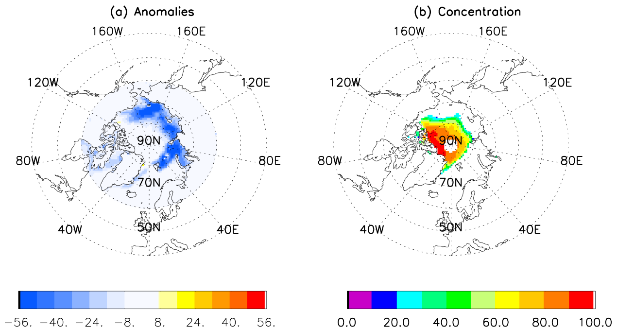
Figure 1 Three-month lead prediction of 2016 September Arctic sea ice concentration anomaly (a) and concentration (b) by the linear Markov model initialized with observed June sea ice concentration, SST and SAT data.
