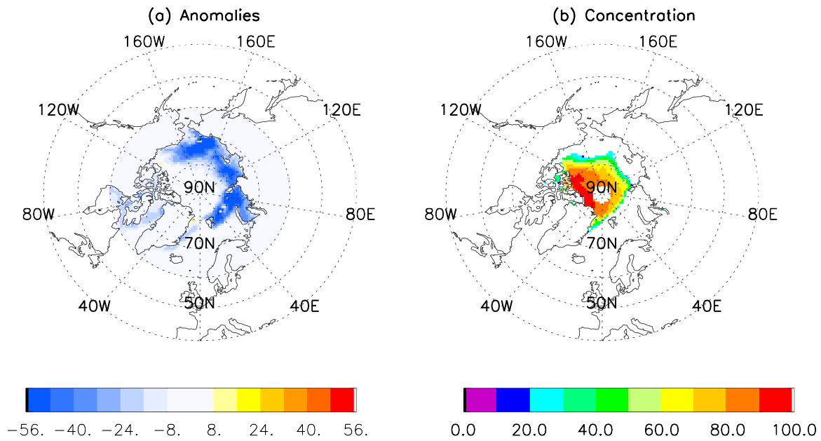
Figure 1 Three-month lead prediction of 2016 September Arctic sea ice concentration anomaly (a) and concentration (b) by the linear Markov model initialized with observed June sea ice concentration, SST and SAT data.
