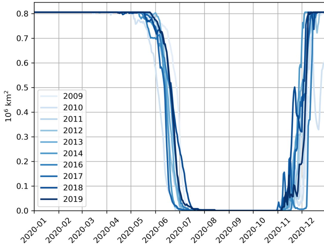
Predicted sea ice extent in region Hudson with various forcing years
