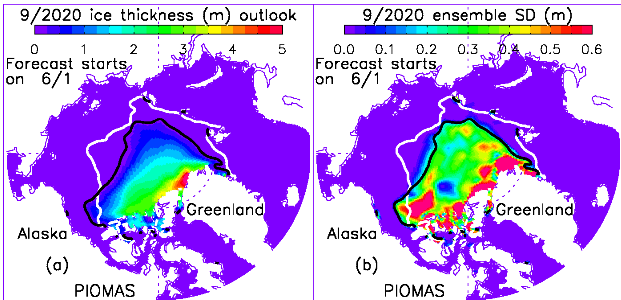
Figure 1. (a) Predicted Arctic September 2020 sea ice thickness and edge location (from ensemble mean), and (b) ensemble standard deviation (SD) of ice thickness which shows the uncertainty of the prediction. The white line represents the satellite-observed September 2018 ice edge defined as the line of 0.15 ice concentration, while the black line is the model predicted September 2020 ice edge.
