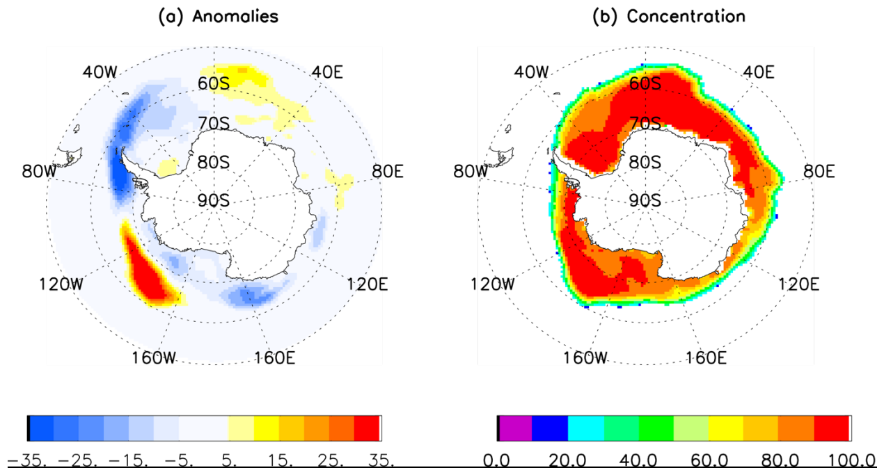
Figure 3 Three-month lead prediction of September 2020 Antarctic sea ice concentration anomaly (a) and concentration (b) by a linear Markov model initialized with observed June SIC, SAT, GH300 and vector winds at 300mb.
