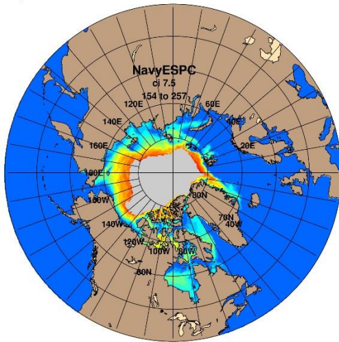
NavyESPC 2020 Jun SIO: Mean First Ice Free Day
