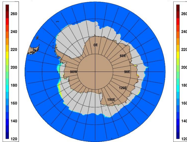
NavyESPC 2020 Jun SIO: Mean First Ice Free Day
