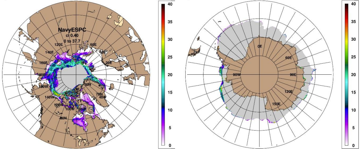
NavyESPC 2020 Jun SIO: Std Dev First Ice Free Day
