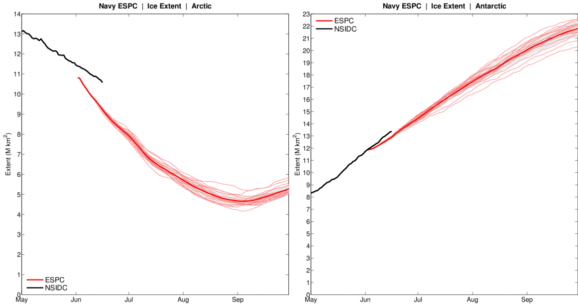
Figure 8: Areal sea ice extent (Mkm 2 ) versus time from the Navy Earth System Prediction Capability 16 member ensemble using 1 June 2020 initial conditions (left – Arctic, right – Antarctic). The thin red curves show the individual members while the thick red curve shows the ensemble mean. The gray shading represents \pm 1 standard deviation. For reference, the thick black curve indicates actual sea ice extent (to date) from the National Snow and Ice Data Center (NSIDC).
