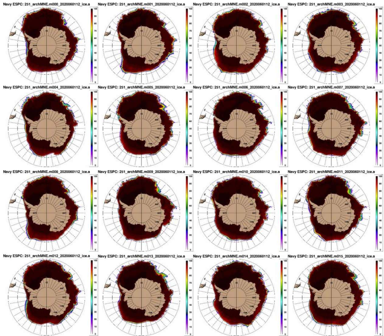
Figure 3: September 2020 mean ice extent from the Navy Earth System Prediction Capability individual 16 members using 1 June 2020 initial conditions for the Antarctic.
