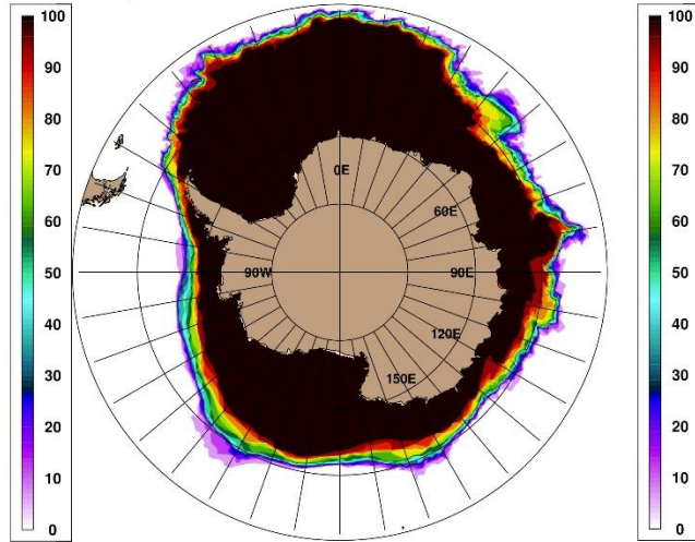
NavyESPC SIP from 1 Jun 2020 IC forecasts
