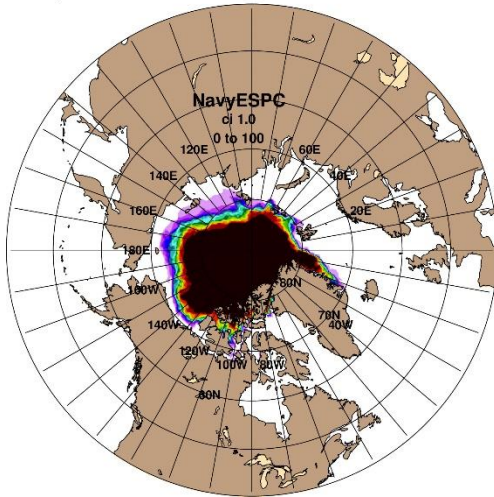
NavyESPC SIP from 1 Jun 2020 IC forecasts
