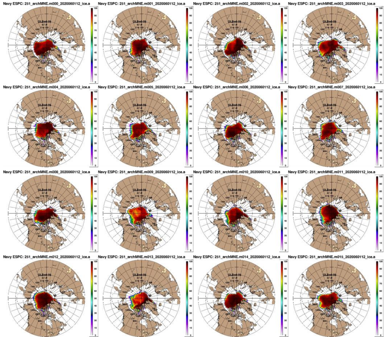
Figure 2: September 2020 mean ice extent from the Navy Earth System Prediction Capability individual 16 members using 1 June 2020 initial conditions for the Arctic.
