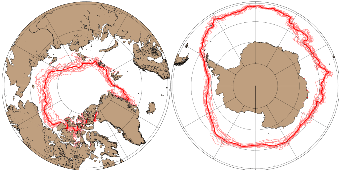
Navy ESPC | Ice Extent | June ICs
