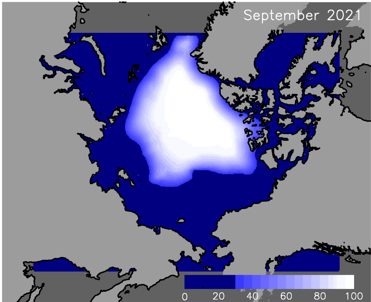
Fig: Predicted monthly-mean ice concentration in September 2021.
