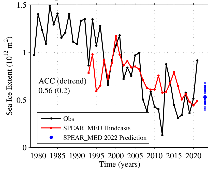
SPEAR_MED September Alaskan Sea Ice Extent Predictions: Jun 1 In
