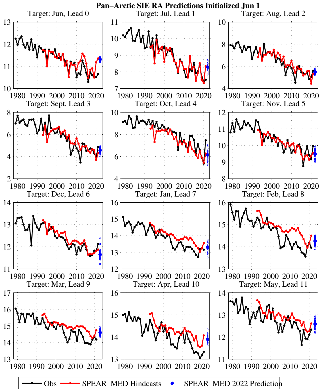
Figure 2: Monthly pan-Arctic sea ice extent predictions from the GFDL-SPEAR_MED model initialized on June 1 (red dots) compared to NSIDC observations (black dots). The blue circles show predictions from the 30 ensemble members. The model predictions have been bias corrected via a linear-regression adjustment.
