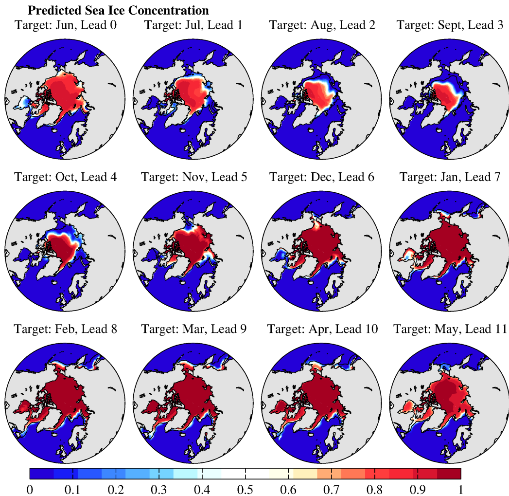
Figure 5: Monthly sea ice concentration predictions from the GFDL-SPEAR_MED model initialized on June 1. The observed climatological sea ice edge position is shown in black. No bias correction has been applied.
