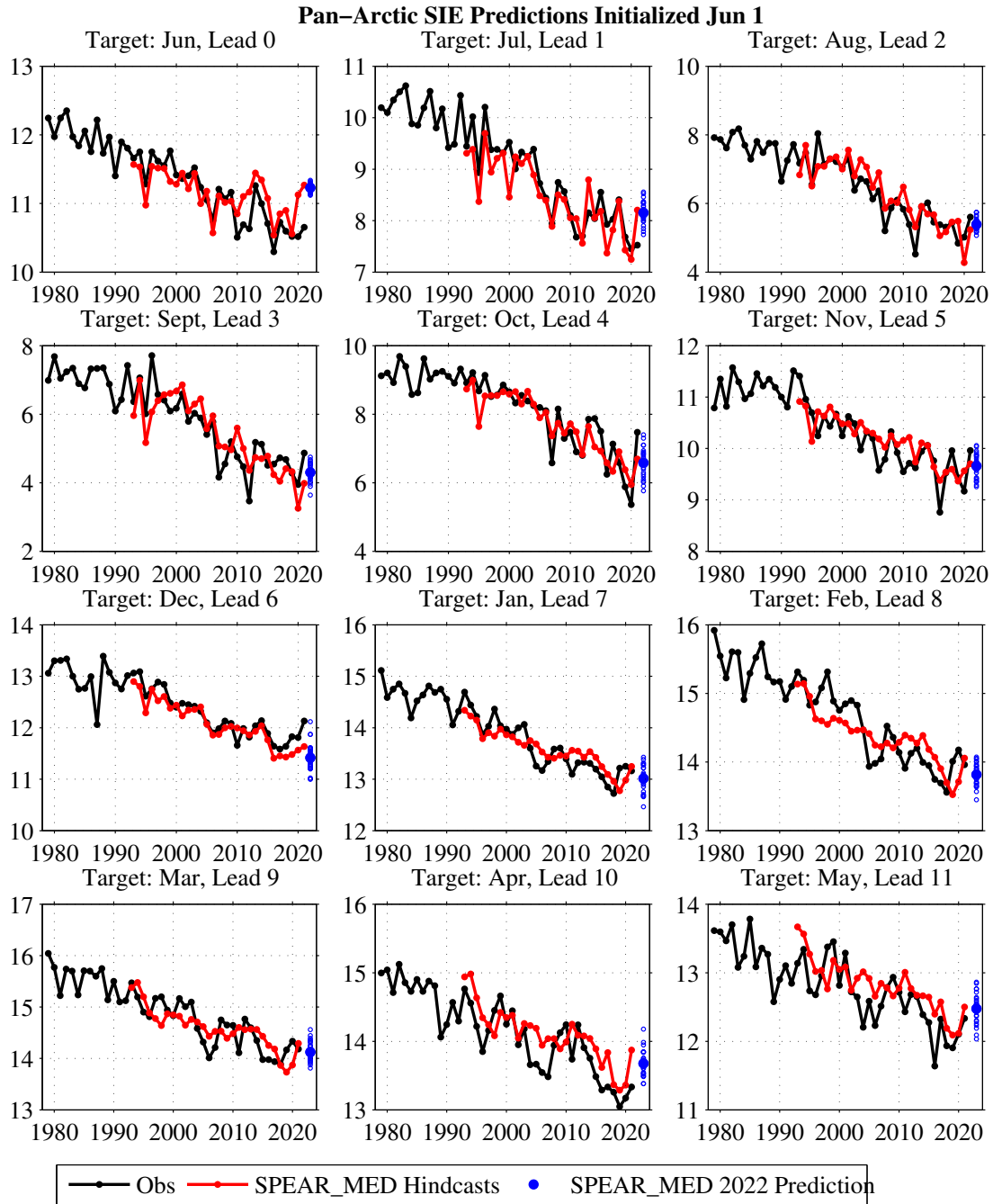
Figure 3: Monthly pan-Arctic sea ice extent predictions from the GFDL-SPEAR_MED model initialized on June 1 (red dots) compared to NSIDC observations (black dots). The blue circles show predictions from the 30 ensemble members. The model predictions have not been bias corrected.
