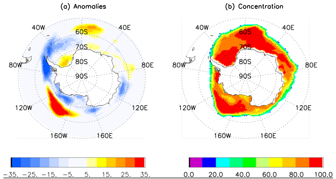
Figure 3 Four-month lead prediction of September 2022 Antarctic sea ice concentration anomaly (a) and concentration (b) by a linear Markov model initialized with observed May SIC, SAT, GH300 and vector winds at 300mb.
