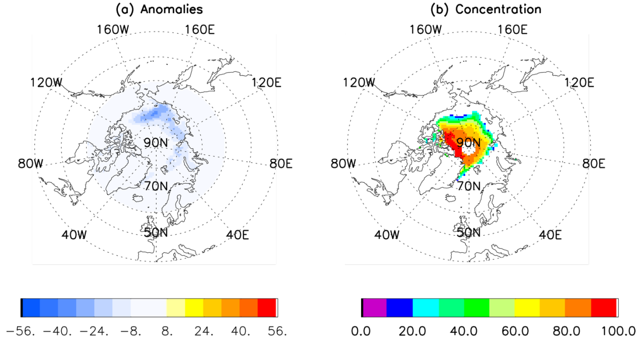
Figure 1 Four-month lead prediction of 2022 September Arctic sea ice concentration anomaly (a) and concentration (b) by the linear Markov model initialized with observed May SIC, SST, SAT, GH300 and vector winds at 300mb.
