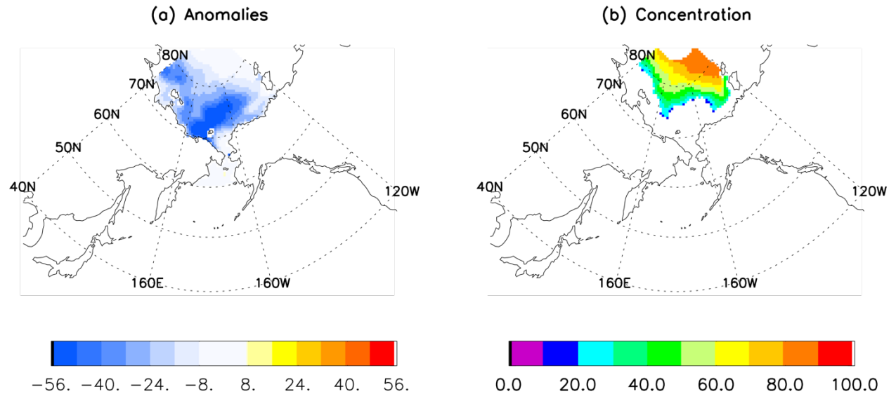
Figure 2 Four-month lead prediction of September 2022 sea ice concentration anomaly (a) and concentration (b) in the Alaskan region by a regional linear Markov model initialized with observed May SIC, SST, SAT, GPH and winds at 500mb and 200mb.
