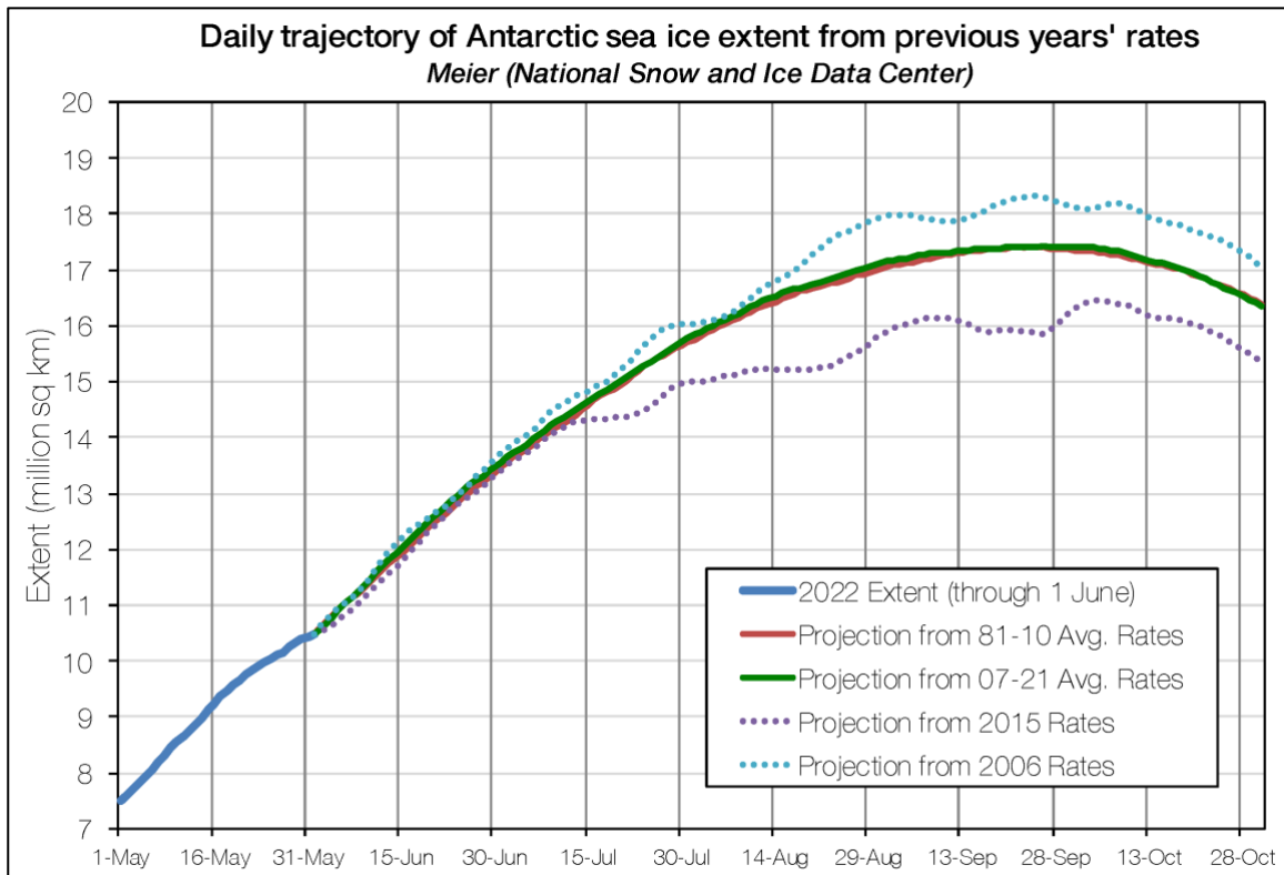
Figure 2. Predicted Antarctic trajectories from the 1 June observed extent. The official estimate is based on the projection used the average of the last 15 years (2007-2021, green solid line) and for the 1981-2010 average (solid red line). The rates for 2006 and 2015 (dotted lines) yield the highest and lowest predicted extents respectively.
