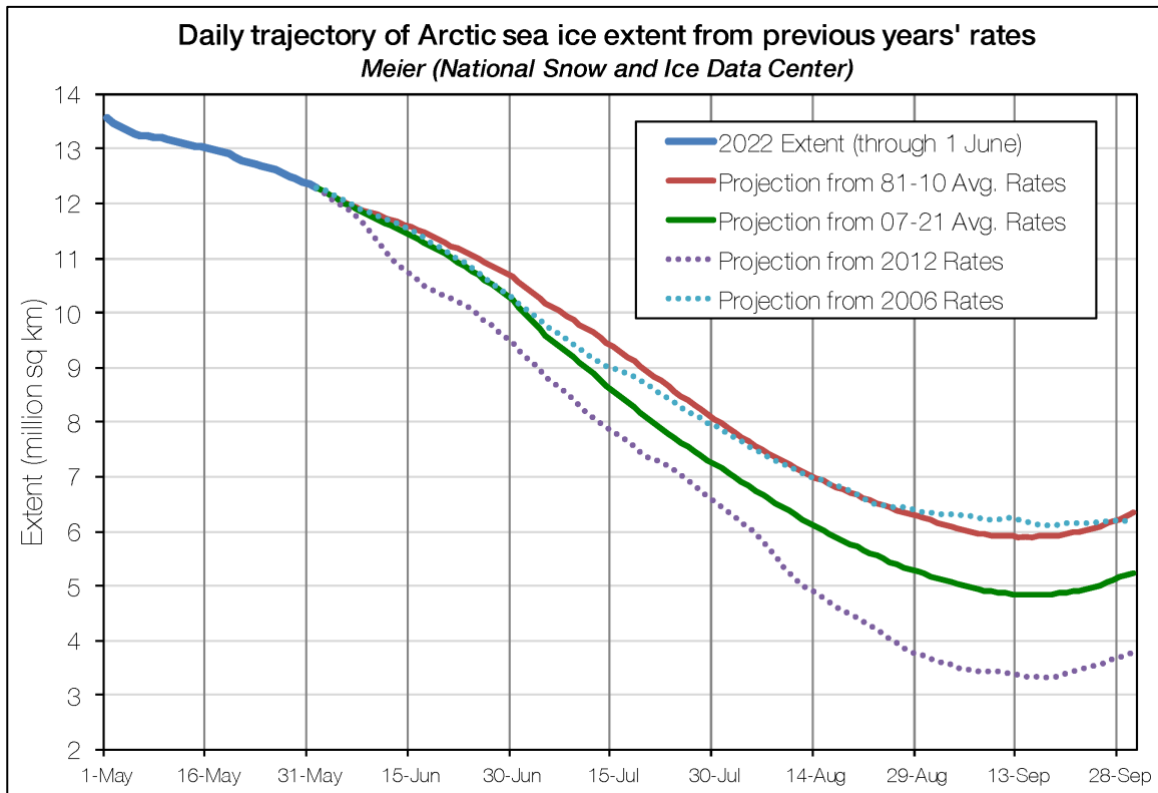
Figure 1. Predicted Arctic trajectories from the 1 June observed extent. The official estimate is based on the projection used the average of the last 16 years (2007-2021, green solid line) and for the 1981-2010 average (solid red line). The rates for 2006 and 2012 (dotted lines) yield the highest and lowest predicted extents respectively.
