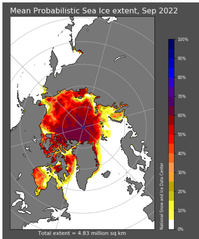
Figure 1: Mean September sea ice extent from Slater Probabalistic Sea Ice Extent Model using May and June data.
