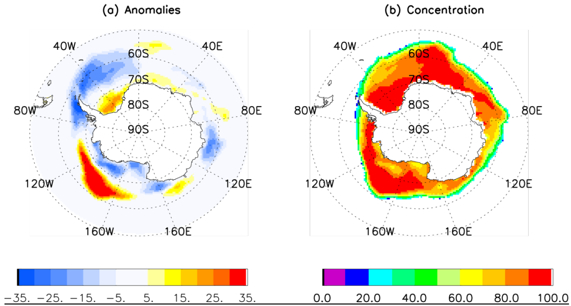
Figure 3 Three-month lead prediction of September 2022 Antarctic sea ice concentration anomaly (a) and concentration (b) by a linear Markov model initialized with observed June SIC, SAT, GH300 and vector winds at 300mb.
