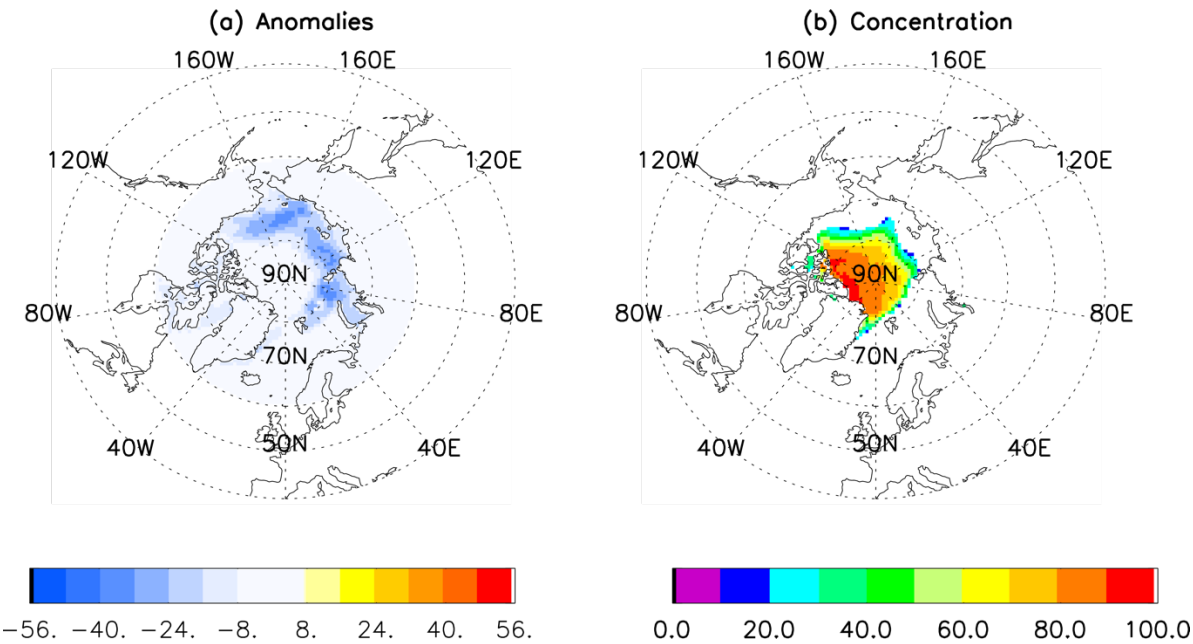
Figure 1 Three-month lead prediction of 2022 September Arctic sea ice concentration anomaly (a) and concentration (b) by the linear Markov model initialized with observed June SIC, SST, SAT, GH300 and vector winds at 300mb.
