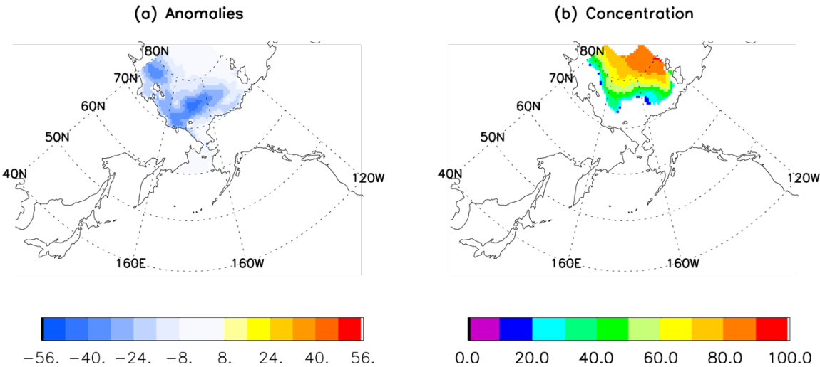
Figure 1 Three-month lead prediction of 2022 September Arctic sea ice concentration anomaly (a) and concentration (b) by the linear Markov model initialized with observed June SIC, SST, SAT, GH300 and vector winds at 300mb.
