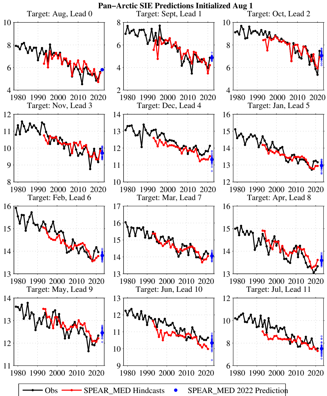
Figure 3: Monthly pan-Arctic sea ice extent predictions from the GFDL-SPEAR_MED model initialized on August 1 (red dots) compared to NSIDC observations (black dots). The blue circles show predictions from the 30 ensemble members. The model predictions have not been bias corrected.
