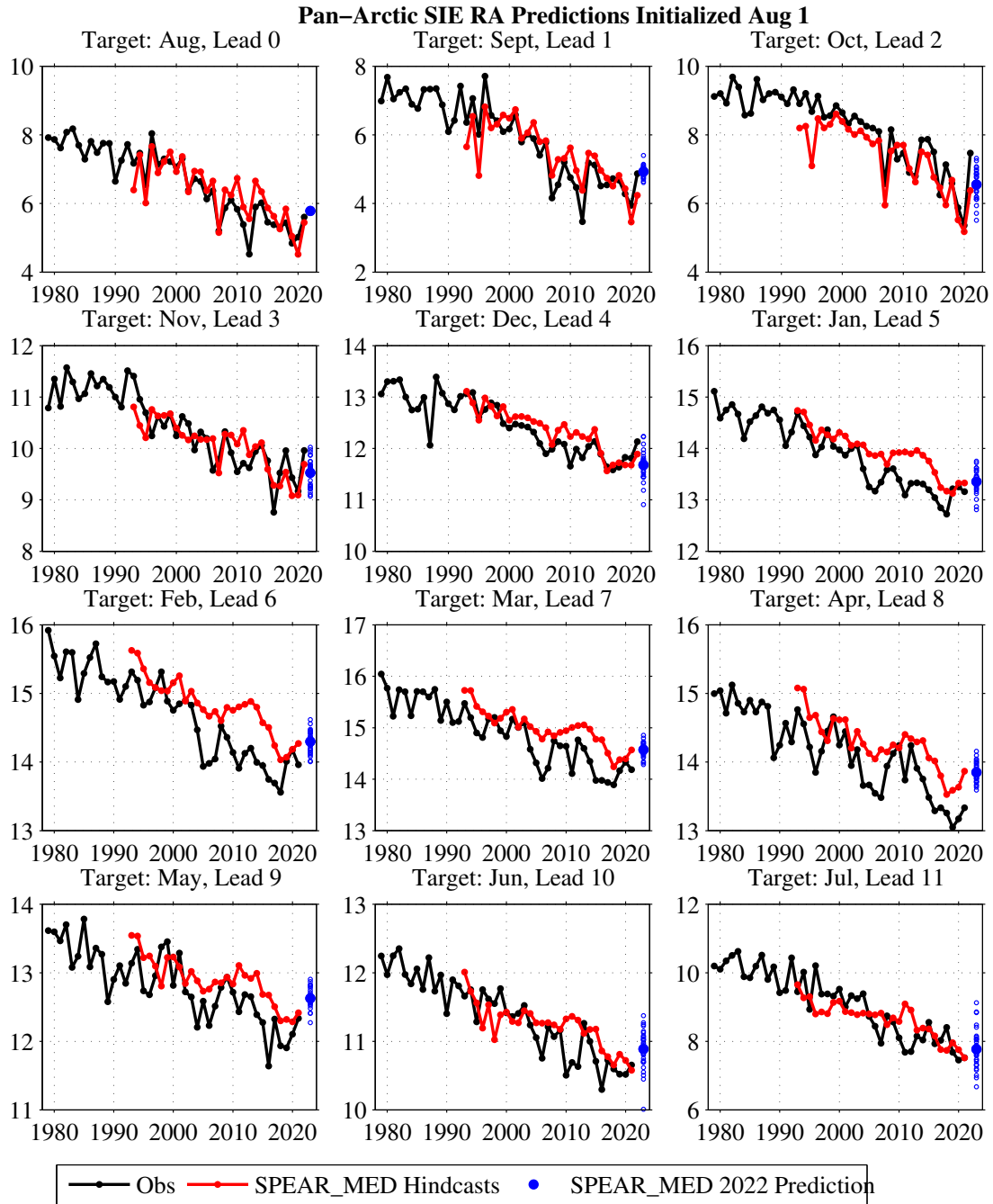
Figure 2: Monthly pan-Arctic sea ice extent predictions from the GFDL-SPEAR_MED model initialized on August 1 (red dots) compared to NSIDC observations (black dots). The blue circles show predictions from the 30 ensemble members. The model predictions have been bias corrected via a linear-regression adjustment.
