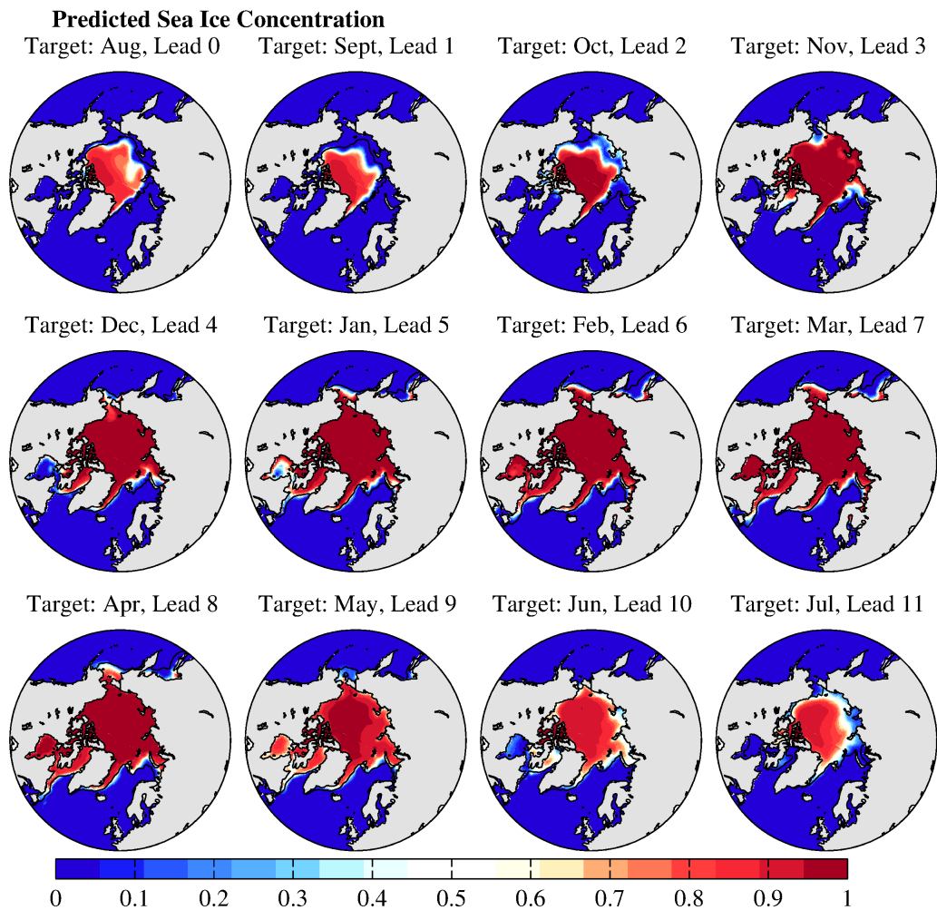
Figure 5: Monthly sea ice concentration predictions from the GFDL-SPEAR_MED model initialized on August 1. The observed climatological sea ice edge position is shown in black. No bias correction has been applied.
