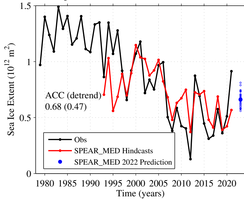
SPEAR_MED September Alaskan Sea Ice Extent Predictions: Aug 1 In
