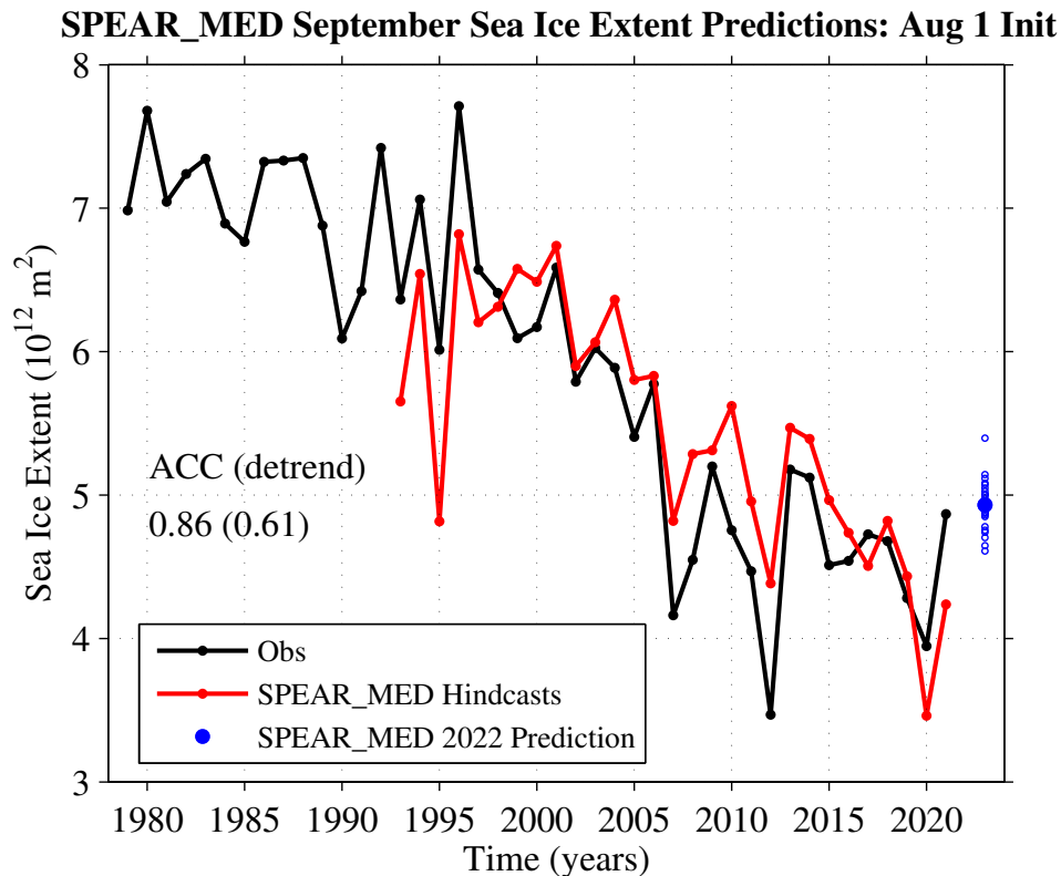
Figure 1: September pan-Arctic sea ice extent predictions from the GFDL-SPEAR_MED model initialized on August 1 (red dots) compared to NSIDC observations (black dots). The blue circles show the September 2022 predictions from the 30 ensemble members. The model predictions have been bias corrected via a linear-regression adjustment.
