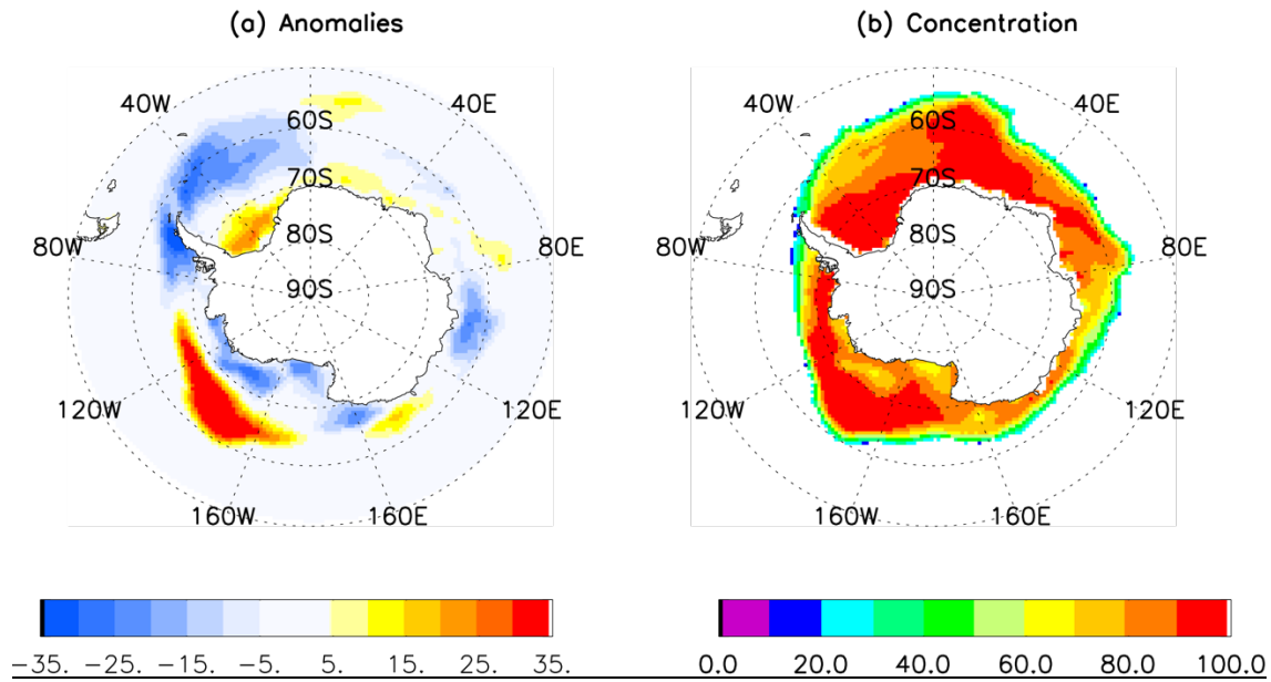
Figure 3 Two-month lead prediction of September 2022 Antarctic sea ice concentration anomaly (a) and concentration (b) by a linear Markov model initialized with observed July SIC, SAT, GH300 and vector winds at 300mb.
