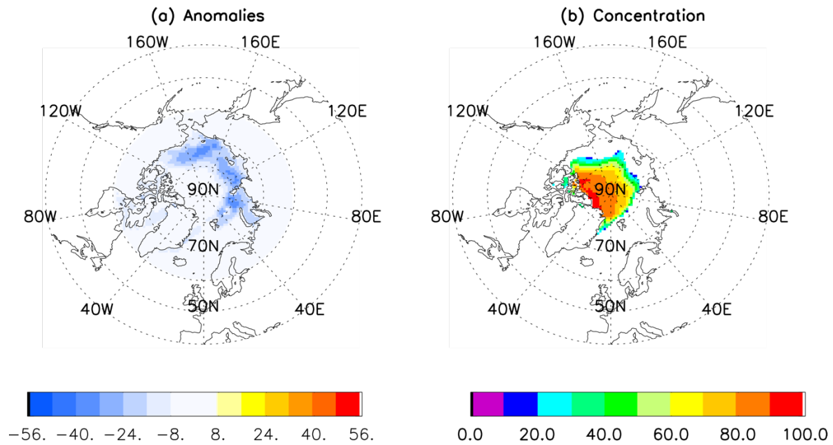
Figure 1 Two-month lead prediction of 2022 September Arctic sea ice concentration anomaly (a) and concentration (b) by the linear Markov model initialized with observed July SIC, SST, SAT, GH300 and vector winds at 300mb.
