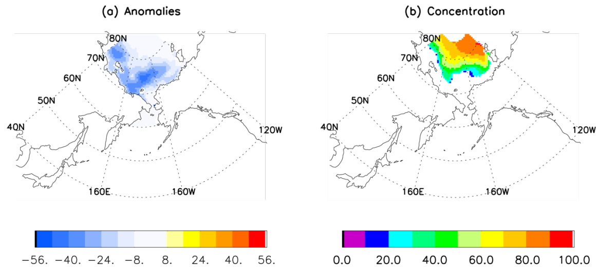
Figure 1 Two-month lead prediction of 2022 September Arctic sea ice concentration anomaly (a) and concentration (b) by the linear Markov model initialized with observed July SIC, SST, SAT, GH300 and vector winds at 300mb.
