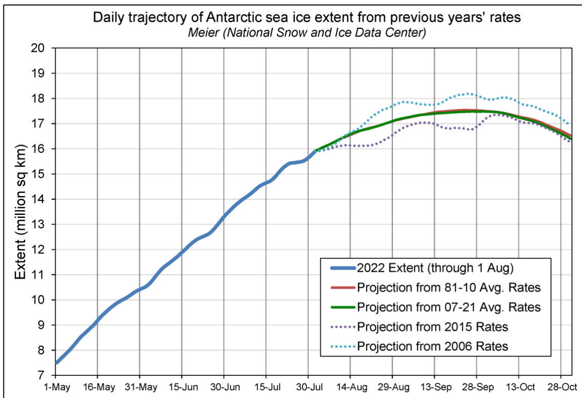
Figure 2. Predicted Antarctic trajectories from the 1 August observed extent. The official estimate is based on the projection used the average of the last 15 years (2007-2021, green solid line) and for the 1981-2010 average (solid red line). The rates for 2006 and 2015 (dotted lines) yield the highest and lowest predicted extents respectively.
