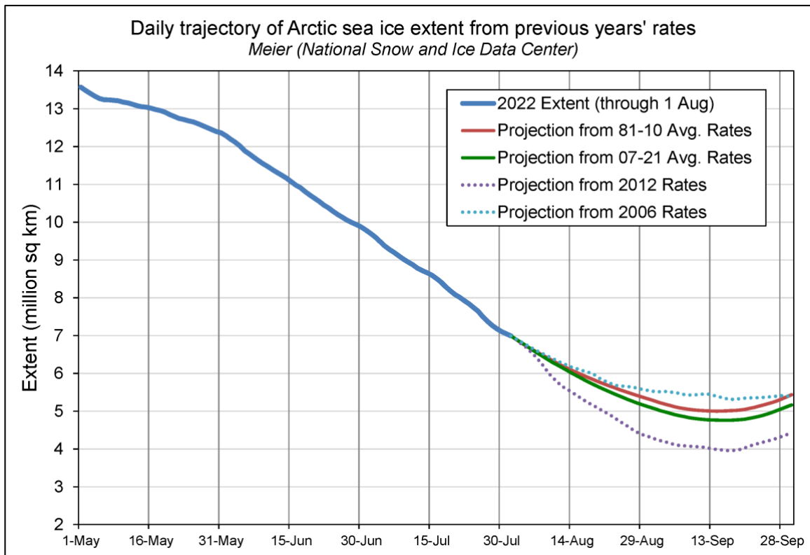
Figure 1. Predicted Arctic trajectories from the 1 August observed extent. The official estimate is based on the projection used the average of the last 15 years (2007-2021, green solid line) and for the 1981-2010 average (solid red line). The rates for 2006 and 2012 (dotted lines) yield the highest and lowest predicted extents respectively.
