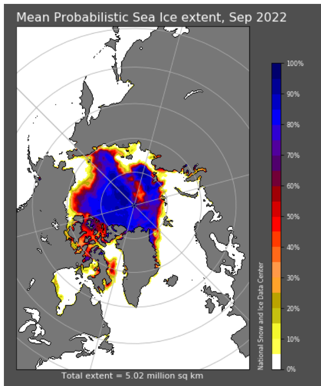
Figure 1: Mean September sea ice extent from Slater Probabilistic Sea Ice Extent Model using May and June data.
