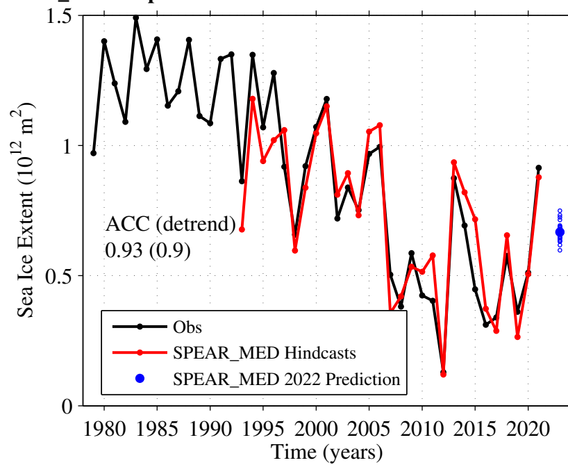
SPEAR_MED September Alaskan Sea Ice Extent Predictions: Sept 1 In
