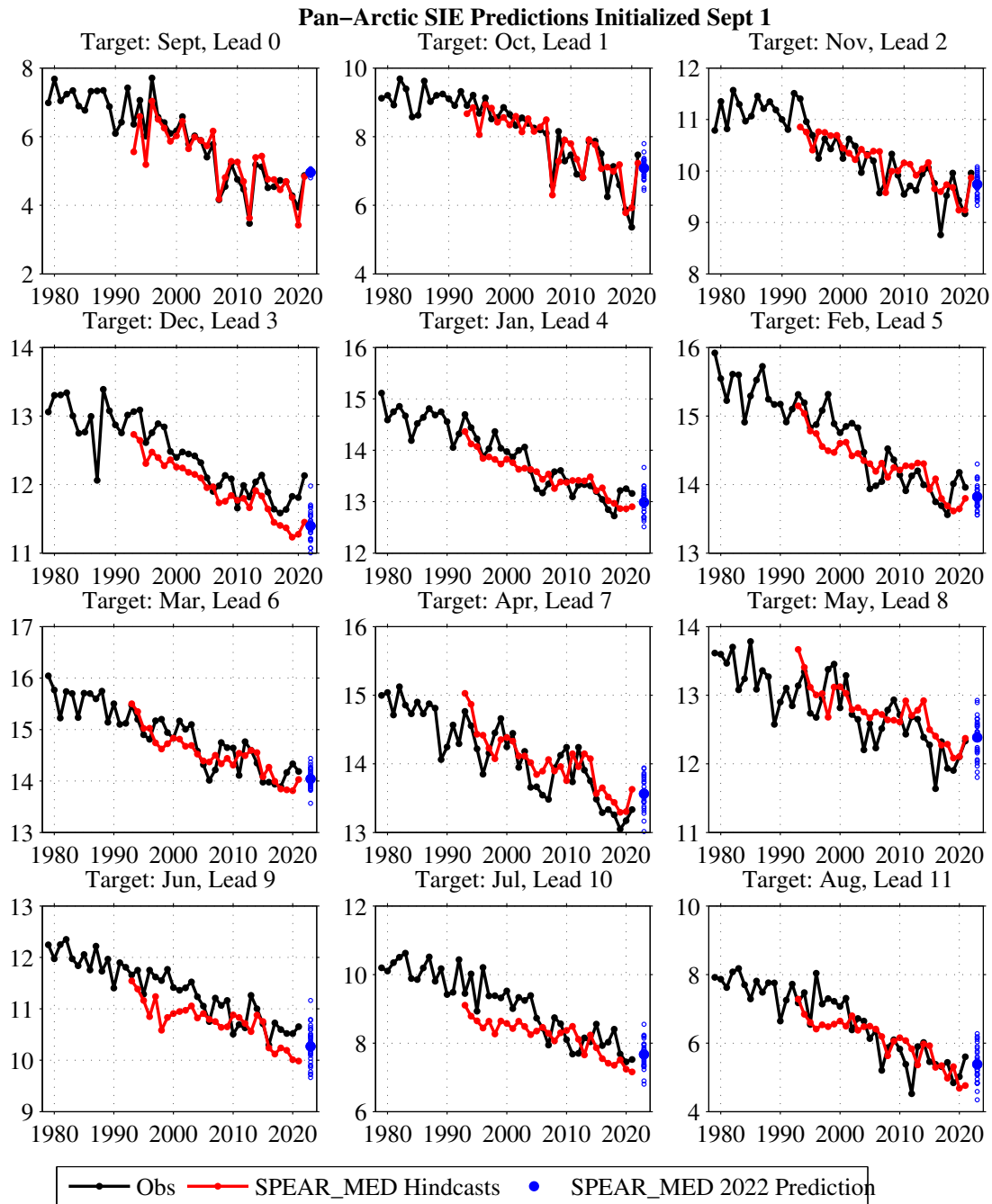
Figure 3: Monthly pan-Arctic sea ice extent predictions from the GFDL-SPEAR_MED model initialized on September 1 (red dots) compared to NSIDC observations (black dots). The blue circles show predictions from the 30 ensemble members. The model predictions have not been bias corrected.
