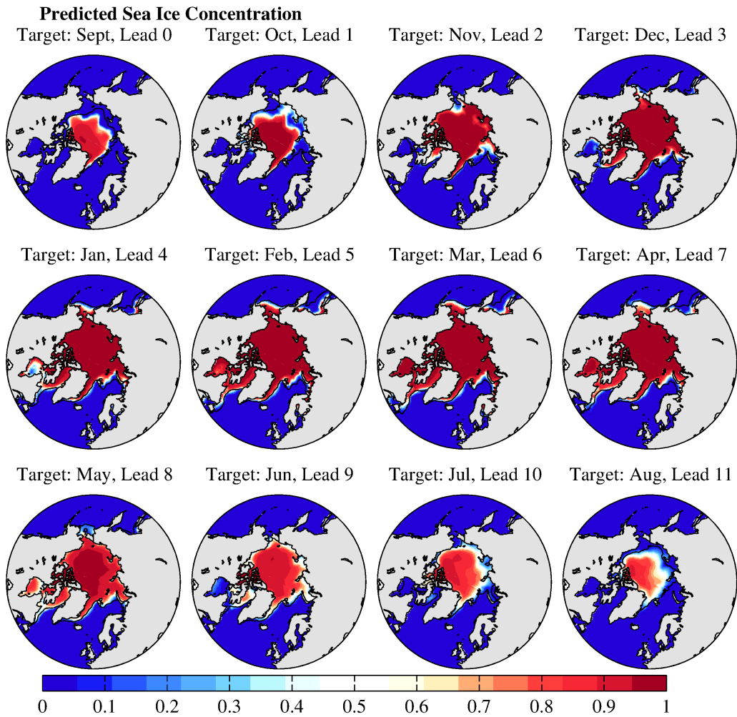
Figure 5: Monthly sea ice concentration predictions from the GFDL-SPEAR_MED model initialized on September 1. The observed climatological sea ice edge position is shown in black. No bias correction has been applied.
