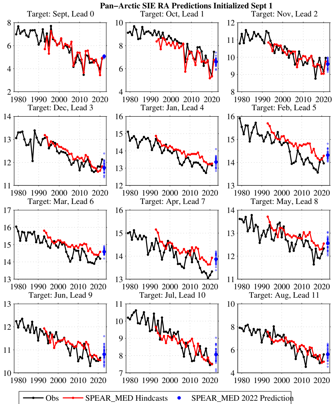
Figure 2: Monthly pan-Arctic sea ice extent predictions from the GFDL-SPEAR_MED model initialized on September 1 (red dots) compared to NSIDC observations (black dots). The blue circles show predictions from the 30 ensemble members. The model predictions have been bias corrected via a linear-regression adjustment.
