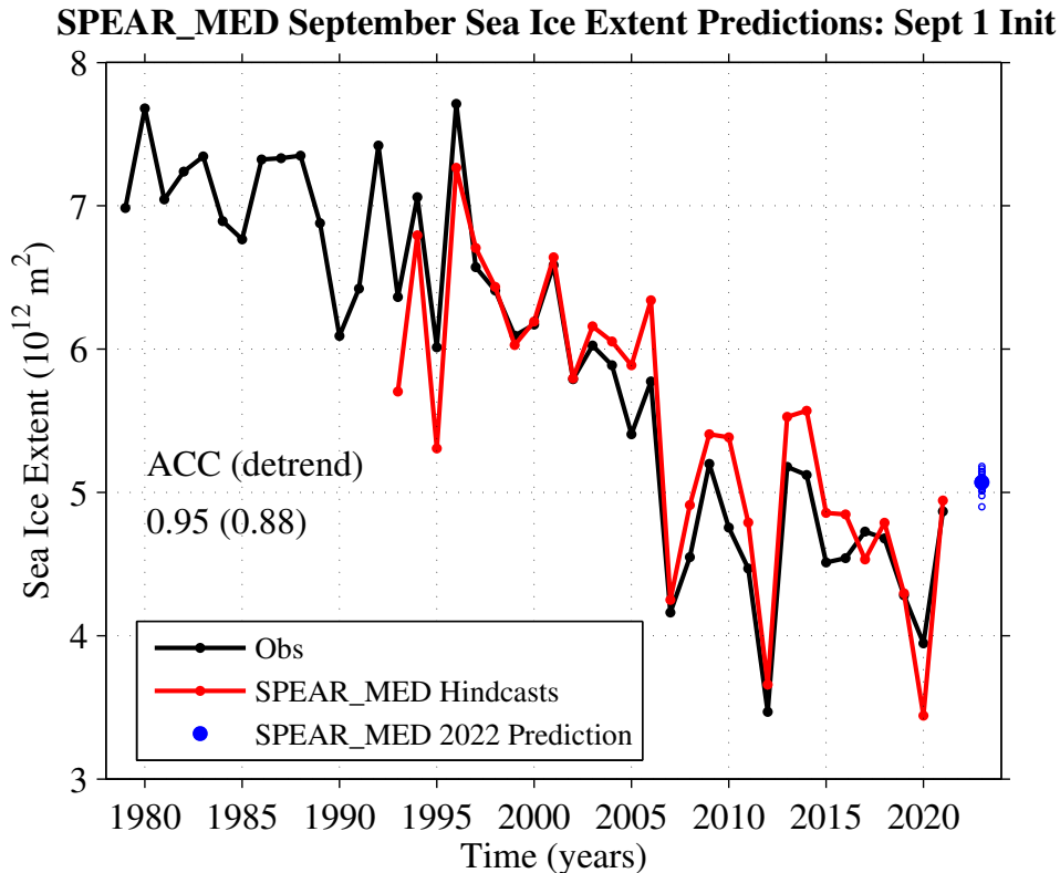
Figure 1: September pan-Arctic sea ice extent predictions from the GFDL-SPEAR_MED model initialized on September 1 (red dots) compared to NSIDC observations (black dots). The blue circles show the September 2022 predictions from the 30 ensemble members. The model predictions have been bias corrected via a linear-regression adjustment.
