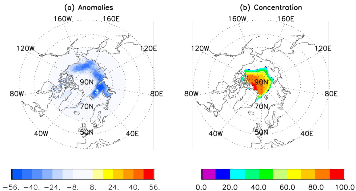
Figure 1 One-month lead prediction of 2022 September Arctic sea ice concentration anomaly (a) and concentration (b) by the linear Markov model initialized with observed August SIC, SST, SAT, GH300 and vector winds at 300mb.
