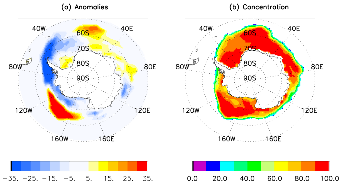
Figure 3 One-month lead prediction of September 2022 Antarctic sea ice concentration anomaly (a) and concentration (b) by a linear Markov model initialized with observed August SIC, SAT, GH300 and vector winds at 300mb.
