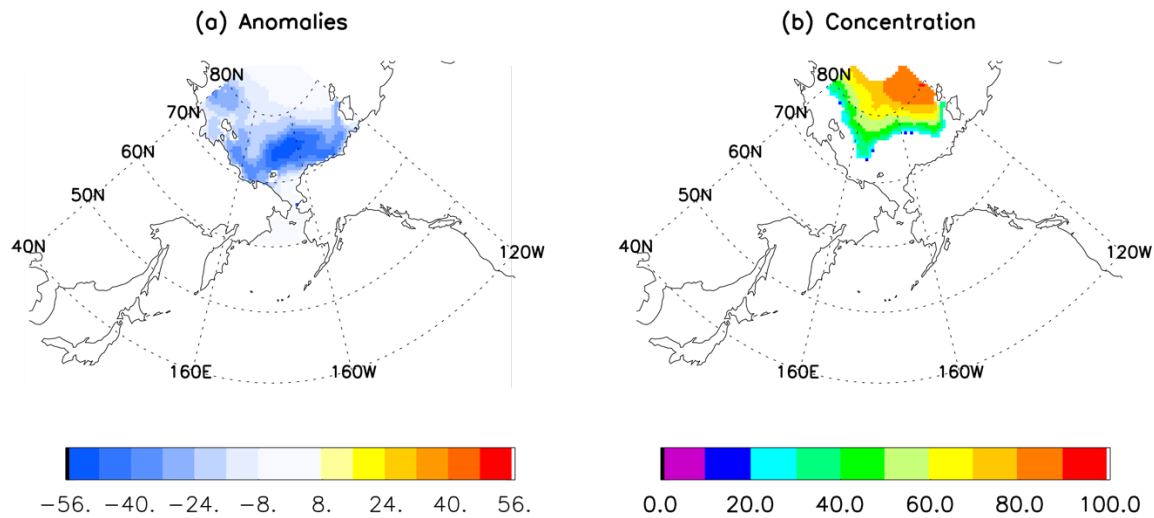
Figure 2 One-month lead prediction of September 2022 sea ice concentration anomaly (a) and concentration (b) in the Alaskan region by a regional linear Markov model initialized with observed August SIC, SST, SAT, GPH and winds at 500mb and 200mb.
